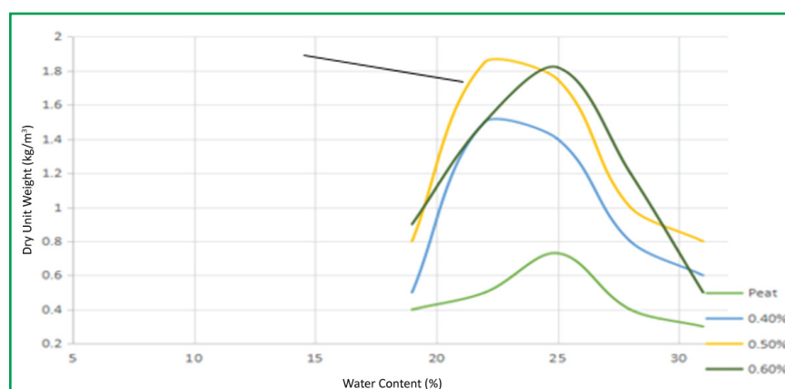
Figure 4. Compaction curve
